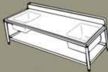
Two Sink Unit Standard Size 60" x 24" x 34" Sink Size 18" x 18" x 10"
